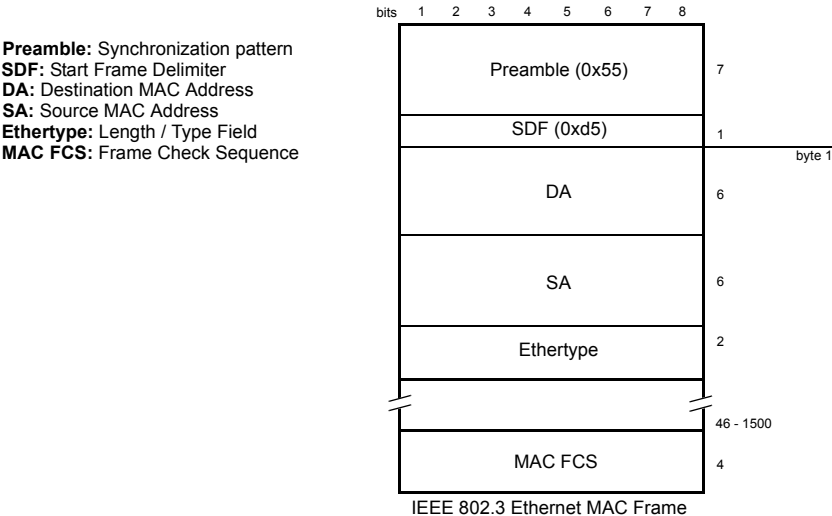
Figure 4.2: IEEE 802.3 frame structure
