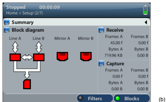
Figure 2.5: Two examples of Net.Shark / Net.Hunter block diagram panel. (a) Connectors and traffic flows when the equipment is configured in Drop mode. (b) Connector usage and traffic flows when the equipment is configured in Capture mode.
