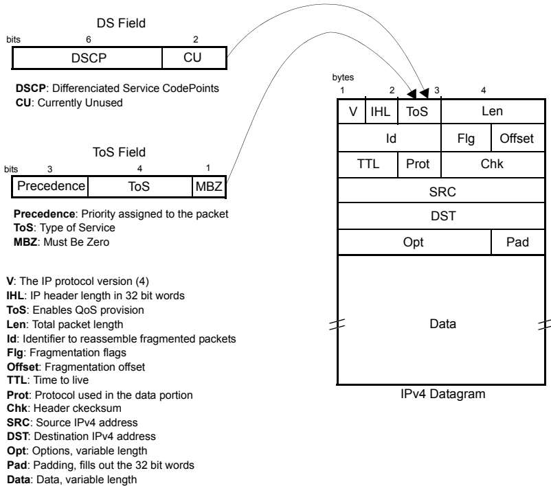
Figure 4.4: IPv4 Datagram structure
